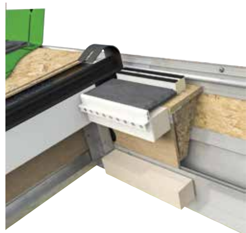
Simplified construction of glazed edge parts
